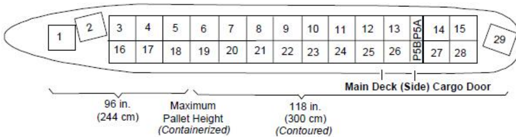
Main Deck 29 Pallets (96 in. x 125 in.) and 2 Half Pallets (96 in. x 53 in.)
